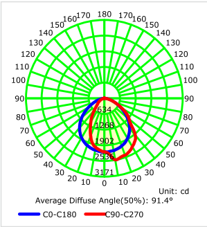
Full cutoff wallpack
