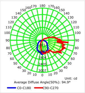
Semi cutoff wallpack
